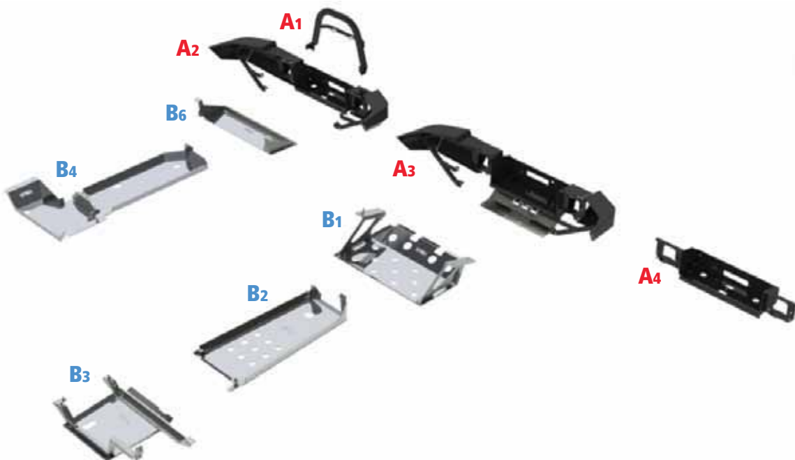
B6 P/N 599077 Radiator & fuel pipes skid plate 06-07 Cannot be mounted with B1
